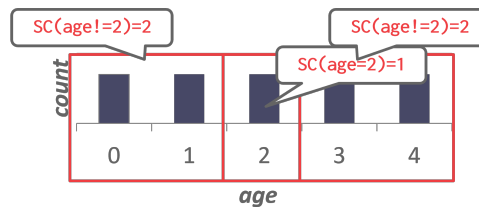
Figure 10: Selectivity of Negation Query Example – The selectivity of the negation query is computed by subtracting the selectivity of the positive query from 1. In the example, the answer comes out to be \frac{4}{5} which is accurate.
