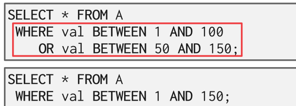
Figure 4: Merging Predicates – The WHERE predicate in query 1 has redundancy as what it is searching for is any value between 1 and 150. Query 2 shows the more succinct way to express request in query 1.
